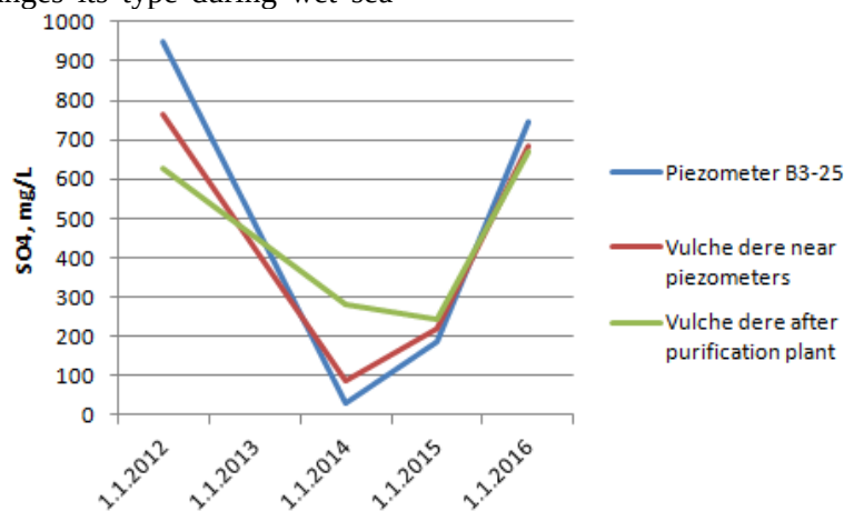
Figure 8: Sulfate concentrations variation over time
