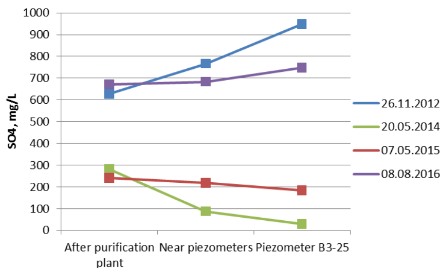
Figure 10: Sulfate concentrations variation along Vulche dere creek and in depth in Quaternary aquifer
