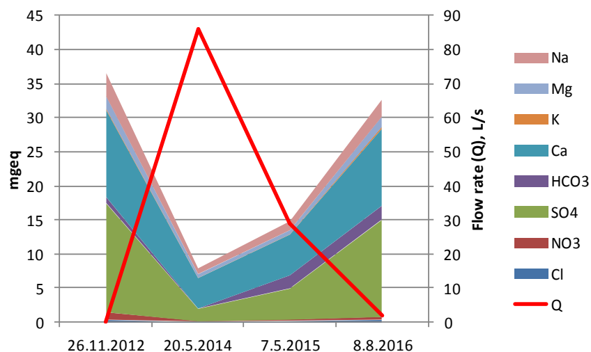
Figure 4: Chemical components and flow rate variation in Vulche dere creek near piezometers
