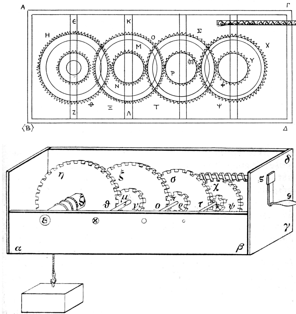
FIGURE 4.2. Weight-lifting reduction gear ( barulkos ) from Heron's Mechanics , as preserved in Greek in his Dioptra . 16 The author explains in detail, referring to the letters in the diagram, how the device allows a force of 5 talents to lift a weight of 1000 talents. Top: diagram as it appears in the Mynas codex (fol. 82r); taken from [Drachmann: MTGRA], p. 25. Bottom: a modern editor's rendition of the same object, based on the textual description and the manuscripts' figures; taken from [Heron: OO], vol. II.1, p. 263. (Manuscript drawings suffer more than the text in the copying process, and important features—here, the gear ratios and the engagement of the endless worm screw on the top right with the wheel—often become corrupt and have to be reconstructed from the text. But the placement of the wheels in the same plane as their axes is a convention motivated by the need to allow easy copying with ruler and compass. For another comparison see page 127.)
