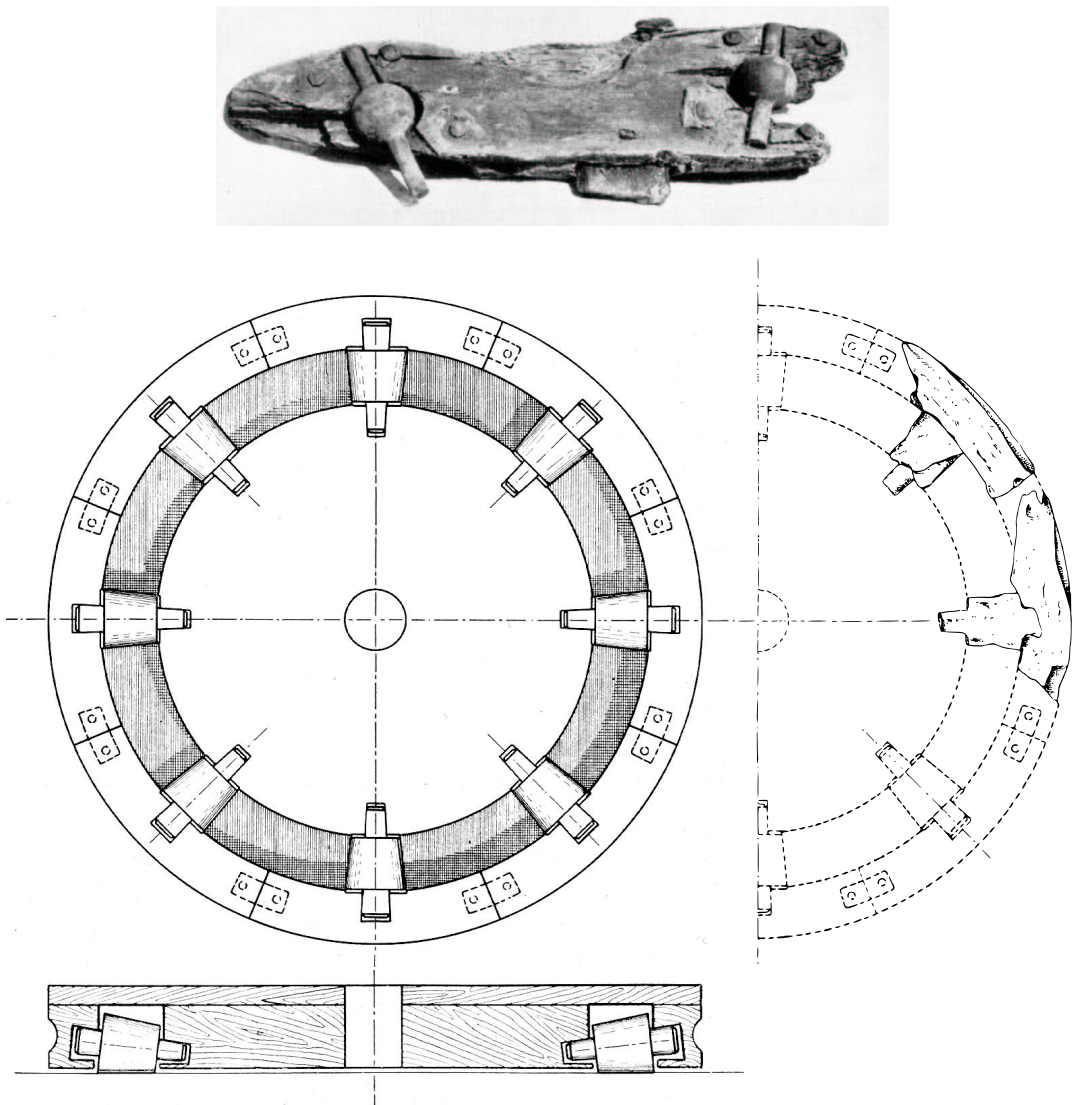
FIGURE 9.4. Brass rollers and remnants of rotating wooden trays encountered in a shipwreck in Lake Nemi and dating from Caligula's time. 96 Top: portion of the rim of a tray about 90cm in diameter. Middle and bottom: reconstruction of another tray with conic rollers. From [Ucelli], pp. 186, 189.
