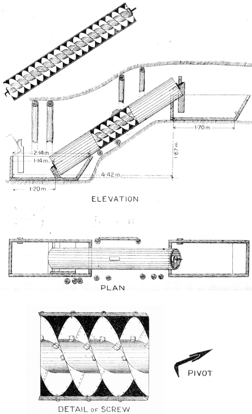
FIGURE 4.9. Roman-time Archimedean screw found at Centenillo Mines, Spain. From [Palmer], p. 330. Scale of plan and elevation, ca. 1:80; details of screw and pivot, ca. 1:20.
