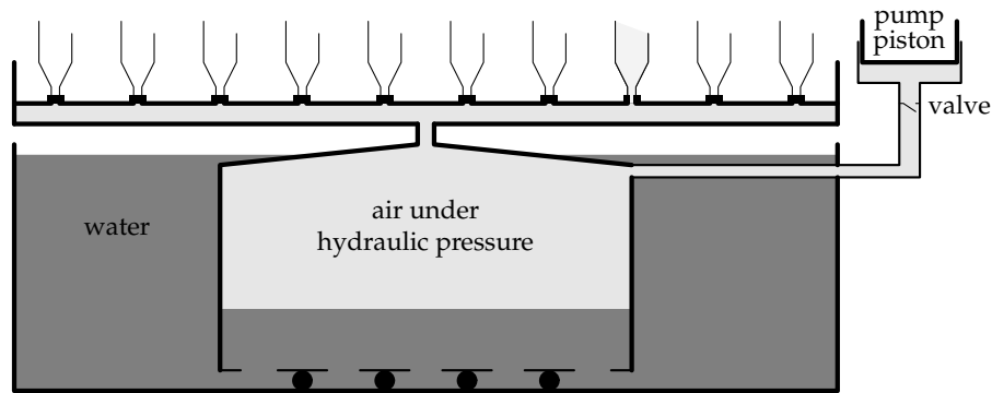
FIGURE 7.10. The Ctesibius water organ as described by Vitruvius and Heron. Based on a drawing of James A. Diamond.
