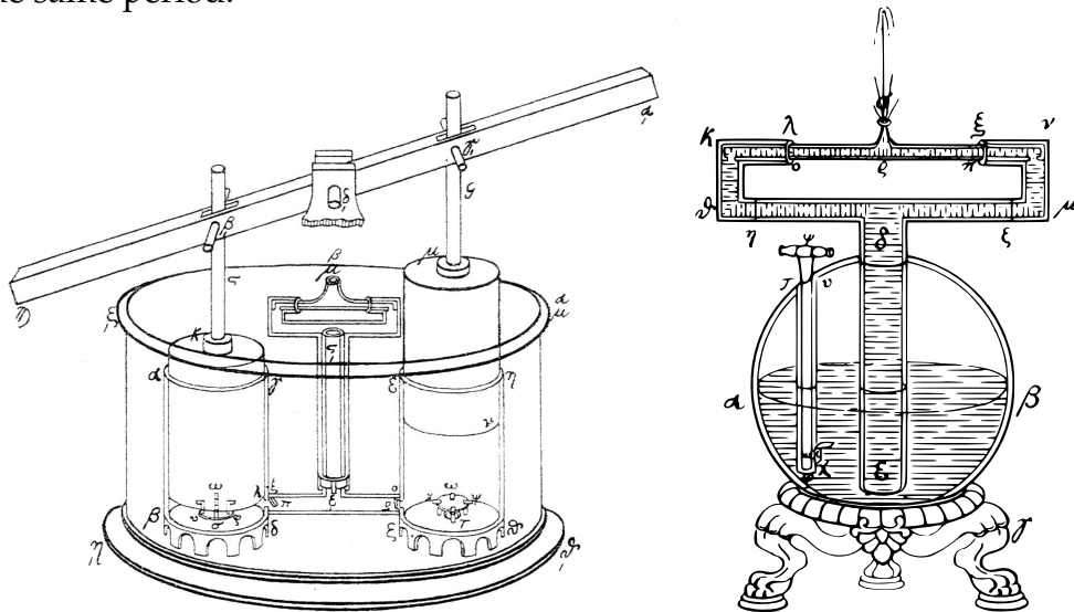
FIGURE 4.15. Two applications of the valve in delivering a jet of water under pressure (Schmidt's redition). Left: The Ctesibian pump configured for use as a fire hydrant, in Heron, Pneumatica , I, xxviii ([Heron: OO], vol. I, p. 133). Right: A Heronian fountain, Pneumatica , I, x ([Heron: OO], vol. I, p. 73).
