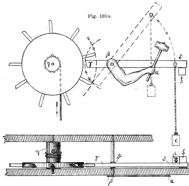
FIGURE 4.16. Detail of an automaton, in Schmidt's rendition. From [Heron: OO], vol. I, p. 425.
