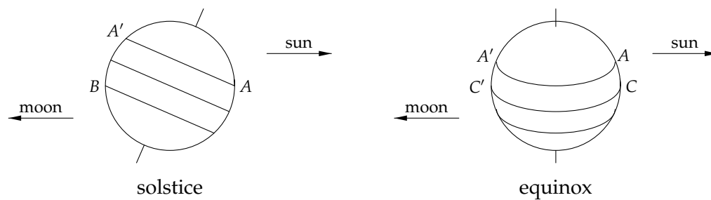
FIGURE 10.5. Configuration of spring tides.
